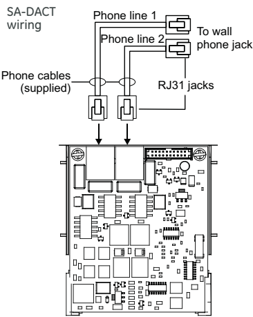
The dialer phone lines connect to connectors on the dialer’s main circuit board. Phone line 1 connects to connector J4 and phone line 2 connects to connector J1.
