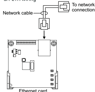
SA-ETH wiring
